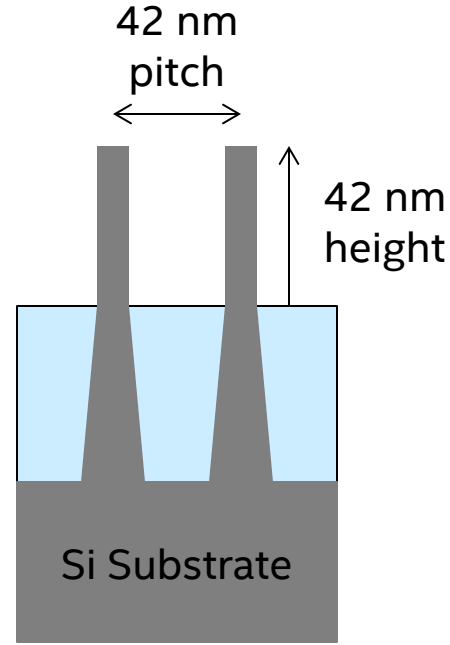
14 nm Process
