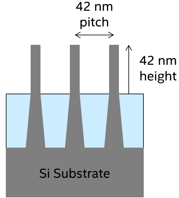
14 nm Process
